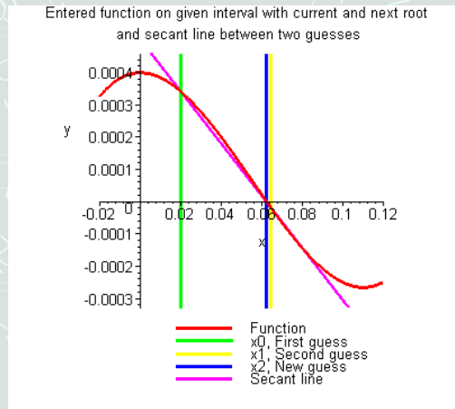
Figure 6 Graph of results of Iteration 2.
