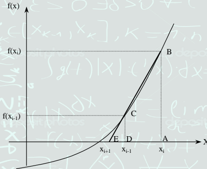
Figure 2 Geometrical representation of the Secant method.
