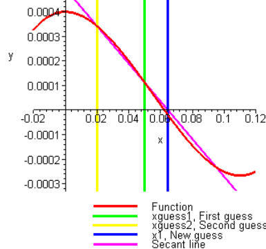
Figure 5 Graph of results of Iteration 1.
